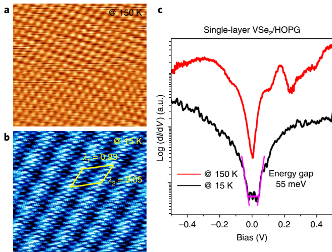
Fig. 2 | Evidence for CDW transition in monolayer VSe 2 . a,b , STM images showing atomic corrugation above the CDW transition (150 K) ( a ) and CDW modulation of atomic corrugation below T_{\text{CDW}} ( b ). In b the CDW unit cell is indicated in yellow together with the approximate periodicities \lambda_1 and \lambda_2 , consistent with previously reported values in ref. 33. STM imaging parameters: V_{\text{bias}} = 700 mV and I_t = 0.6 nA. c , STS shows the opening of an energy gap at low temperatures, which is extracted by the tangential approximation of the differential conductance shown by the pink lines in c .
